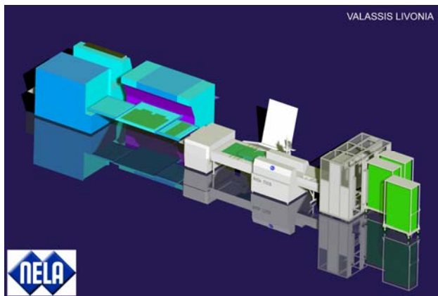
3-D Layout of the installation at Valassis, Livonia, MI
